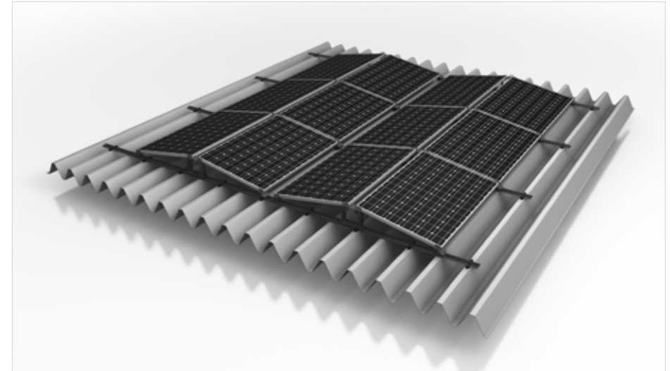
K2 D-Dome System on Trapezoidal sheet
